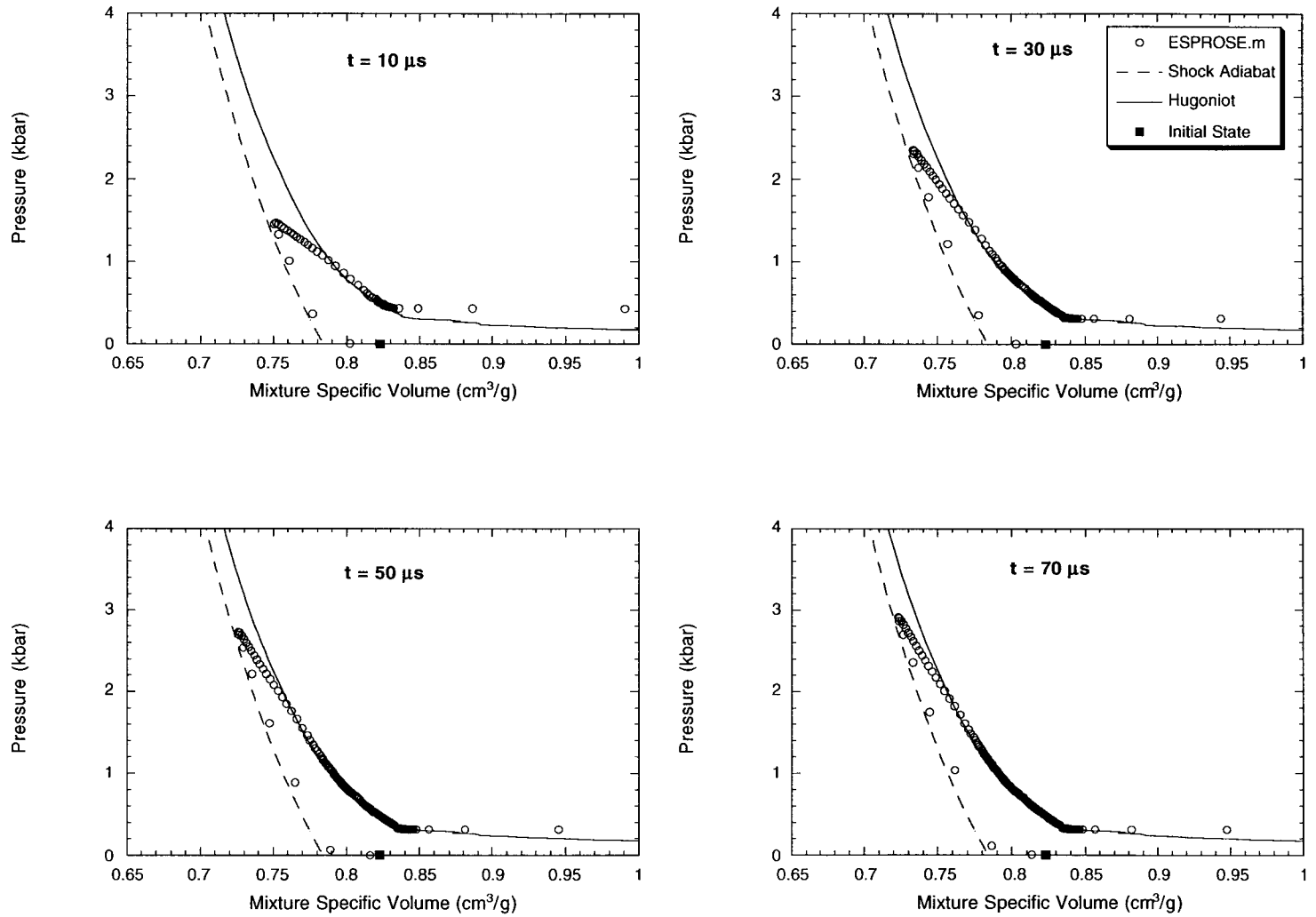
Fig. 11. The ESPROSE.m result at 20 \mu\text{s} intervals in the p-v plane, in relation to the shock adiabat and the Hugoniot.
