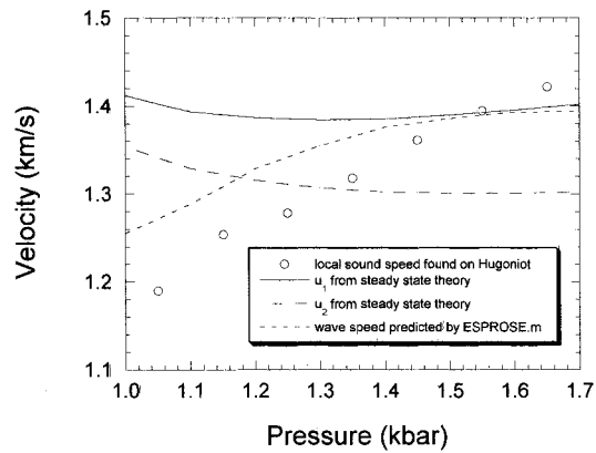
Fig. 12. Demonstration of choking at the C–J point as predicted by the steady state theory and the wave speed of the ESPROSE.m solution.
