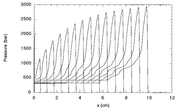
Fig. 10. Illustration of escalation and approach to steady state propagation in an ESPROSE.m simulation of a tin (1500°C)–water explosion, with a premixture void fraction of 5% and fuel fraction of 5%. Print interval is 5 \mu s.
